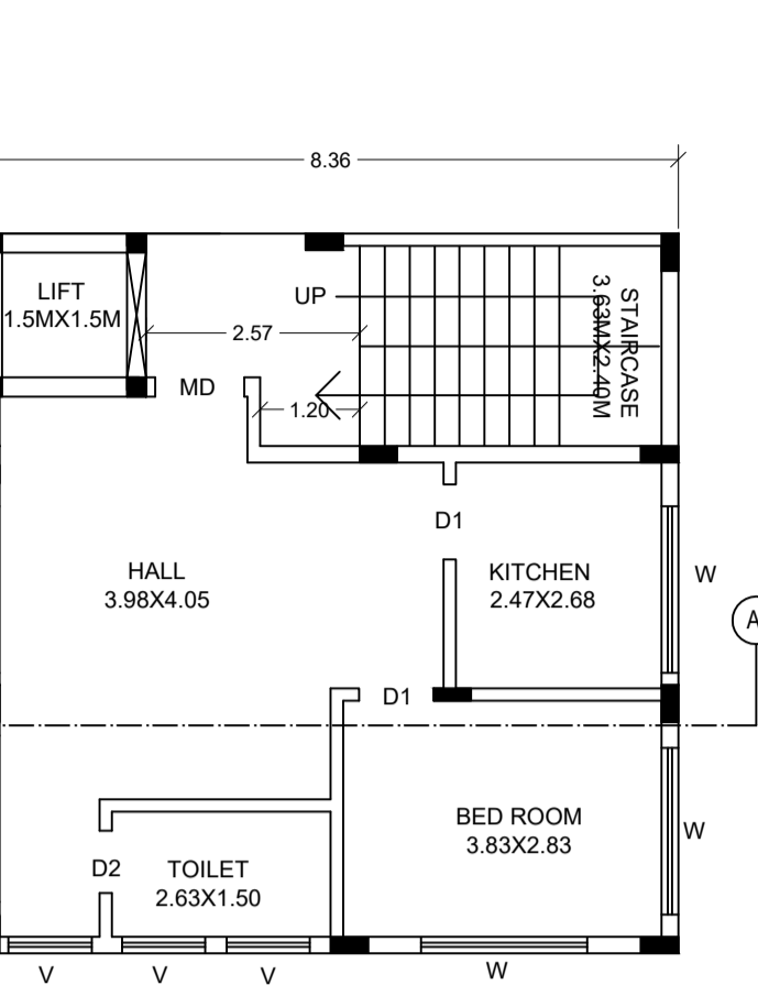
PROPOSED TYPICAL-GROUND FLOOR & FIRST FLOOR PLAN
